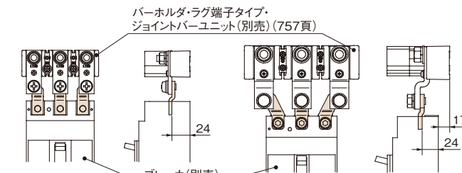
[BP34-LT615W・1525W取付例]
